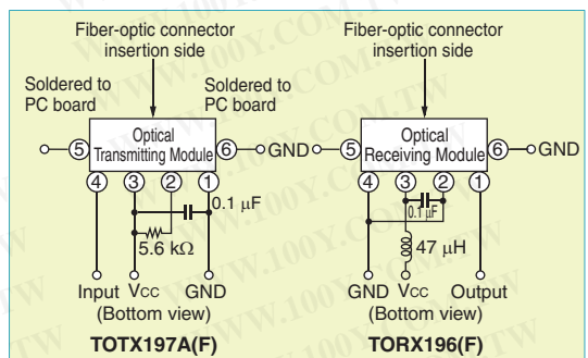
Application circuits for the TOTX197A(F) and TORX196(F)
