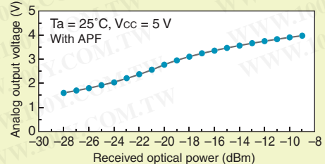
Receiving module with an analog output for optical flux monitoring
